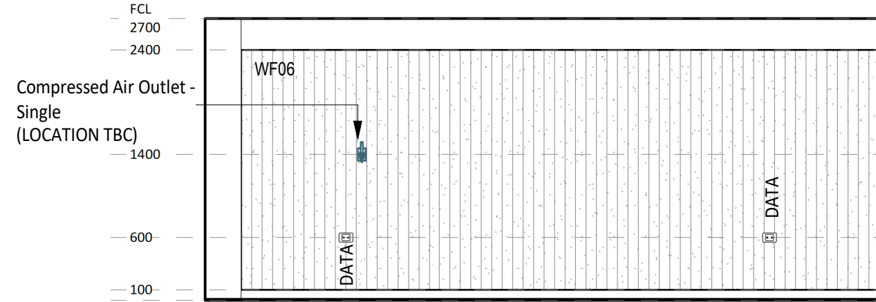
5 ELEVATION DETAIL 60-019 1 : 50
