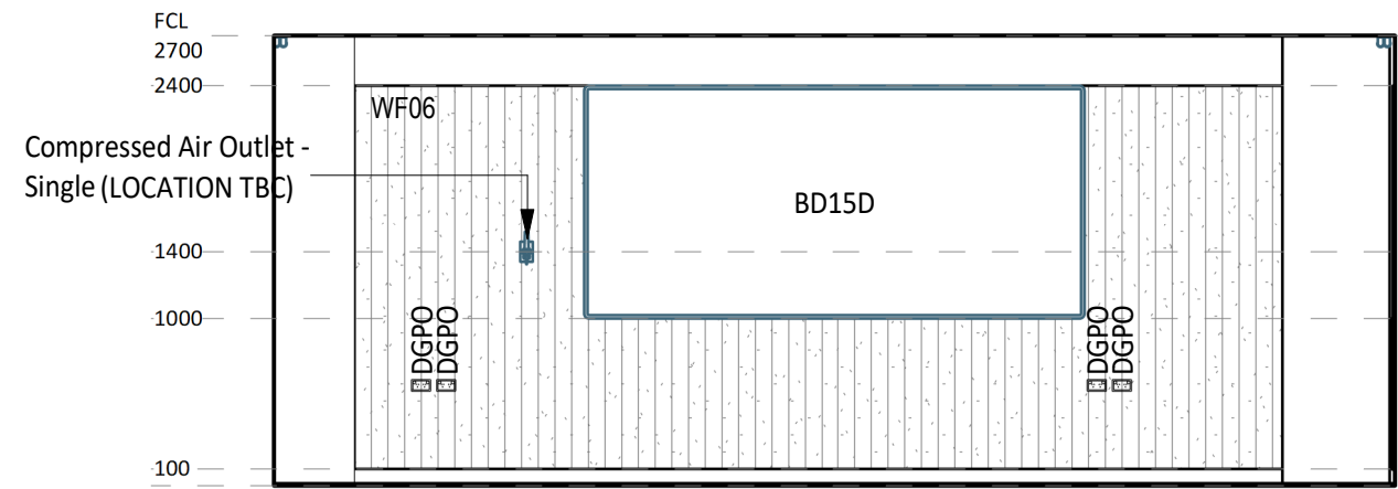
3 ELEVATION DETAIL 60-019 1 : 50
